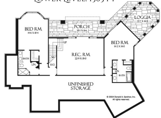
LOWER LEVEL: 1363 FT 2
